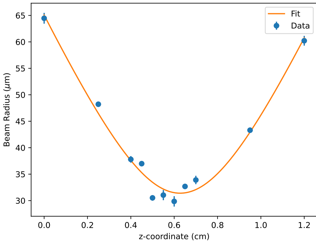
z-coordinate vs. Beam Radius
